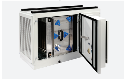
Main filter consisting of ioniser and collector
